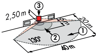
RC-plus next 130
