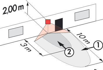
FL3N-LED-130
