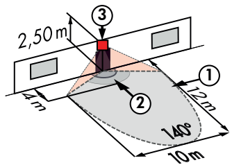
LC-Mini 120
