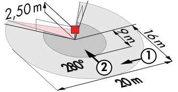
LC-plus 280
